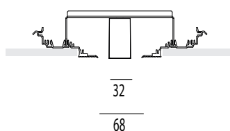
STAFFA MINIFILE BRACKET MINIFILE
