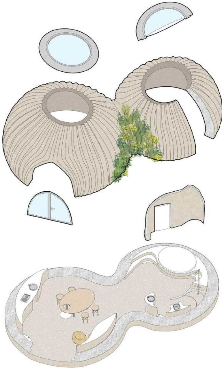
TECLA3D Printed House Assonometria
